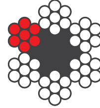
6x7 STD
