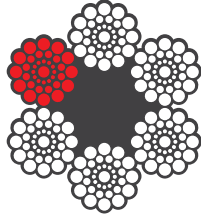
6x31 WS
