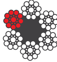
6x26 WS
